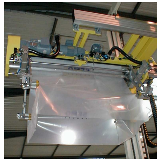
Opening and rotation of the hood for 1/2 and crosswise pallets
